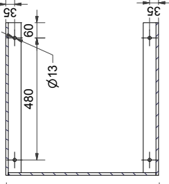
E-E ( 1:10 )
